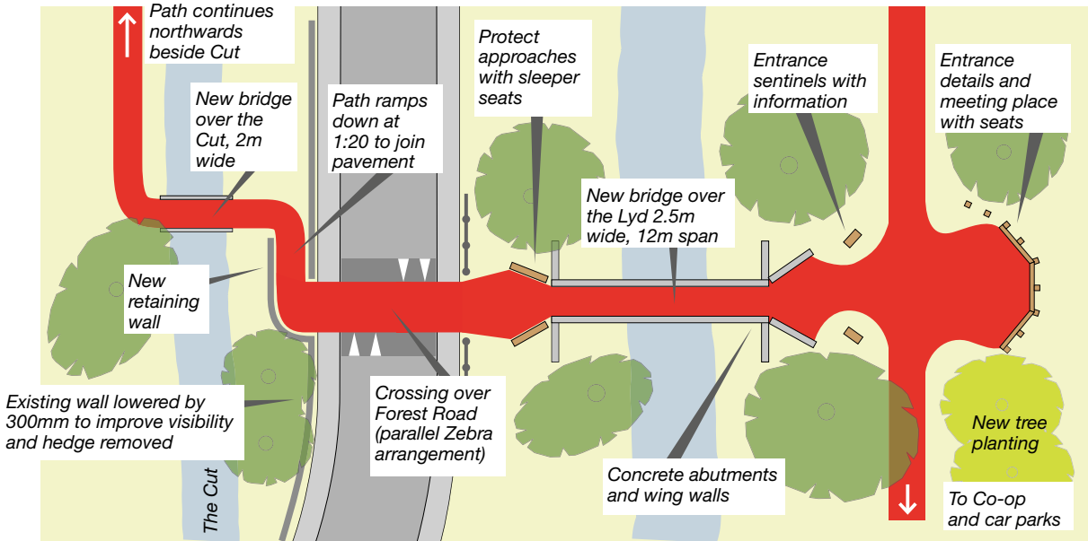
GH4 Plan of ramp down from Cut and raised pavement over the road through to Co-op path
