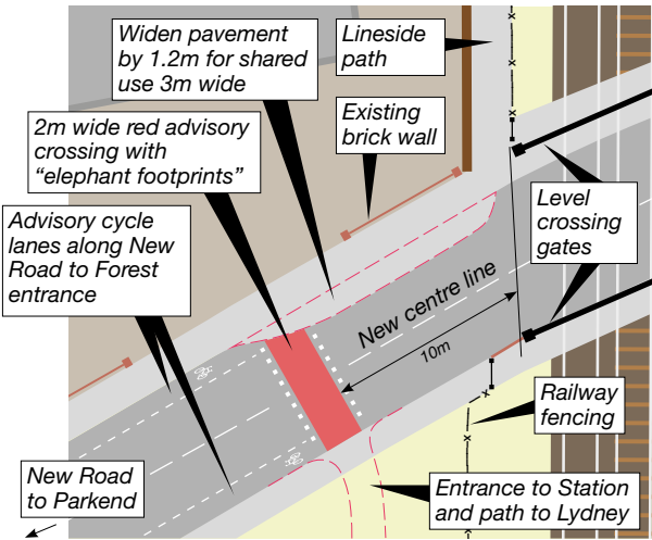
Plan of proposed crossing of New Road at Whitecroft
