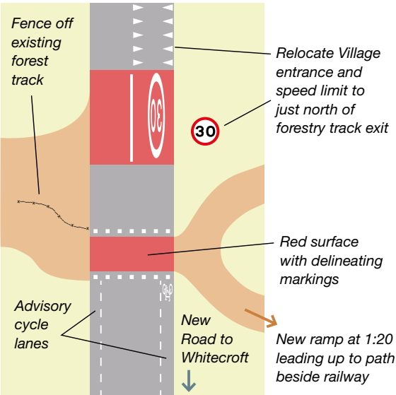
FE5 Crossing New Road: This sketch is also GH1 Gloucestershire Highways
