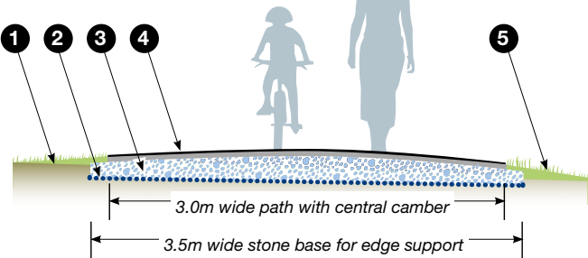
Cross section through 3m wide path
